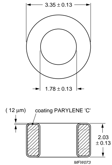
Fig.1 TC3.4/1.8/2 ring core.
