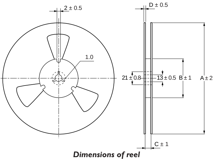
MLS-MLP-MLN Dimensions in mm
