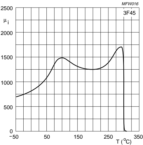
Fig.2 Initial permeability as a function of temperature.
